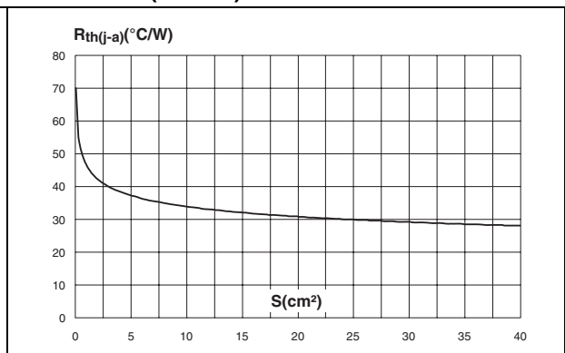
Figure 12. Thermal resistance junction to ambient versus copper surface under tab (epoxy printed board FR4, copper thickness = 35 \mu\text{m} ) (D 2 PAK)
